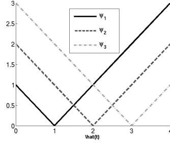
Figure 3: The surrogate \psi
